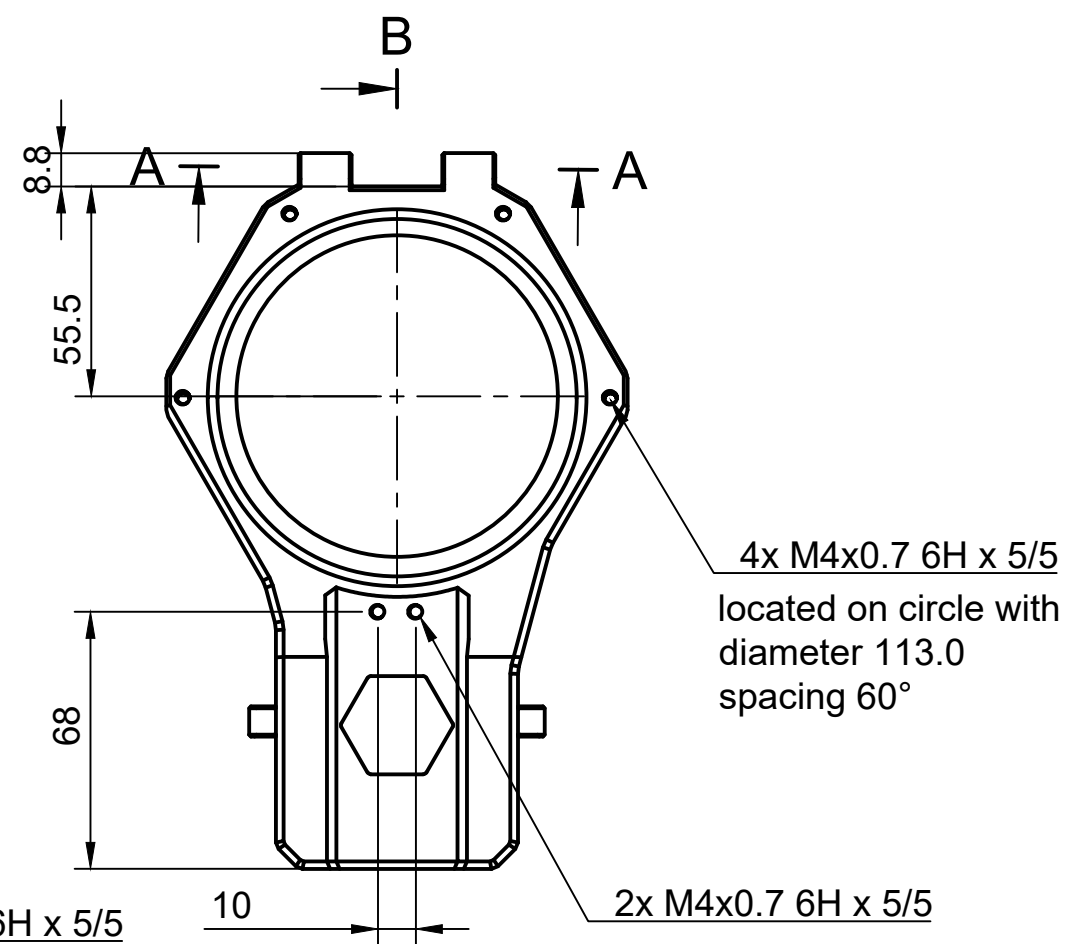
Front View (1:2)
