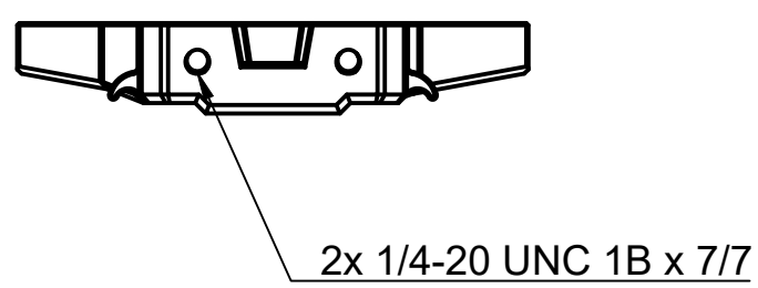
Bottom View (1:2)
