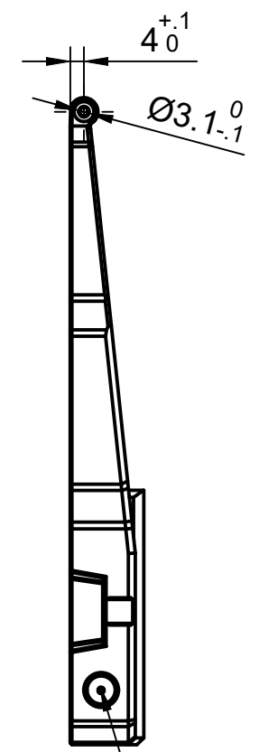
Side View (1:2)
